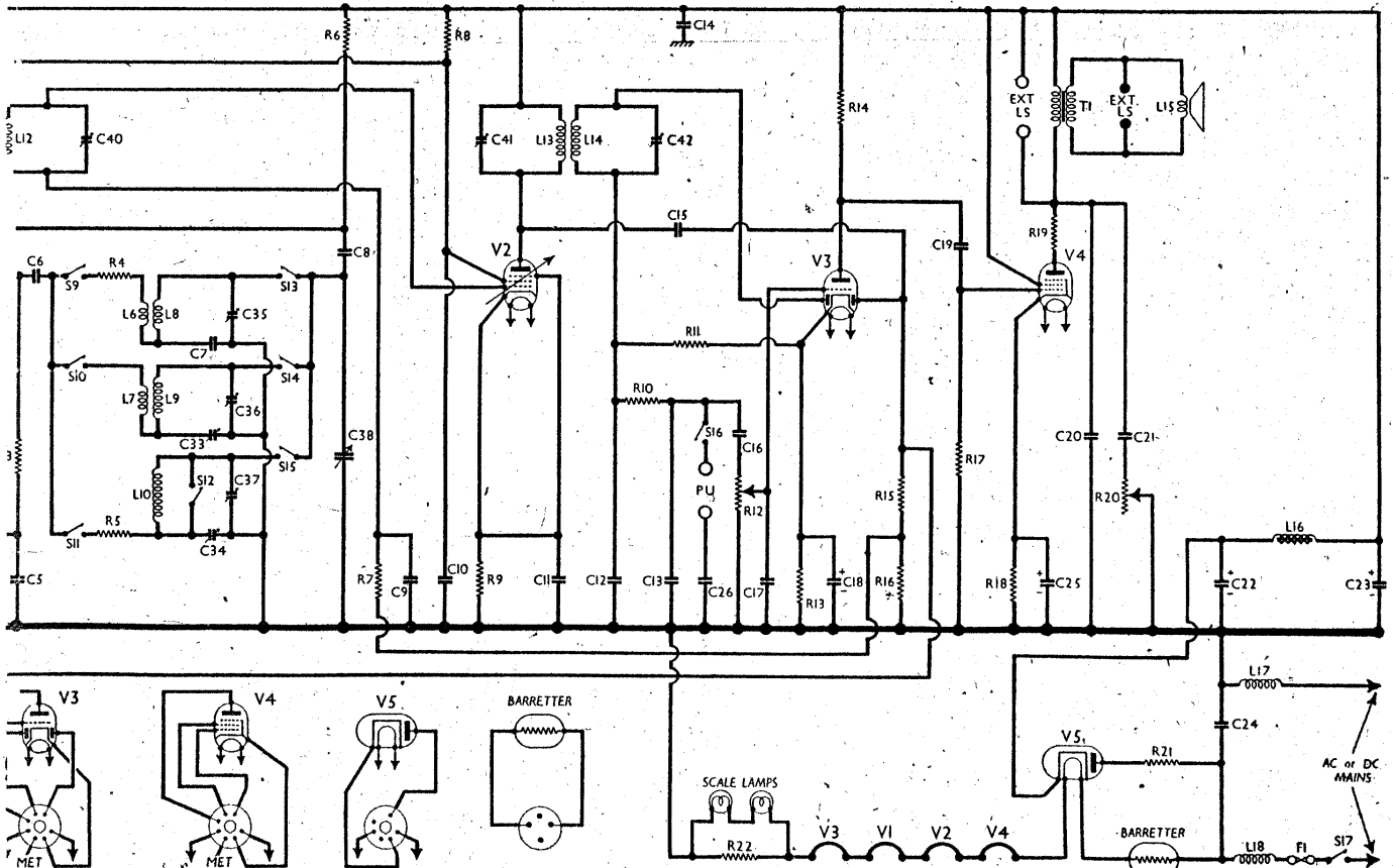
superhet. The differences in the export models are fully explained overleaf, and the diagram there can be made to overlap this one.
