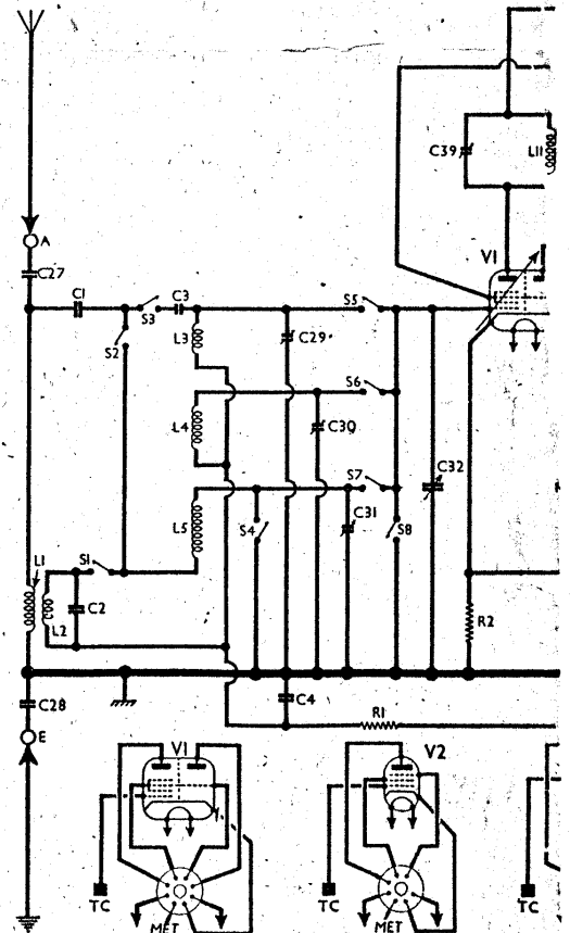
Circuit diagram of the Ferguson 101U AC/DC
